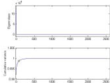
Figure 1. The distribution of variance, where ‘o’ denotes that the largest 75 variances are up to 99.8% of all the variance.
