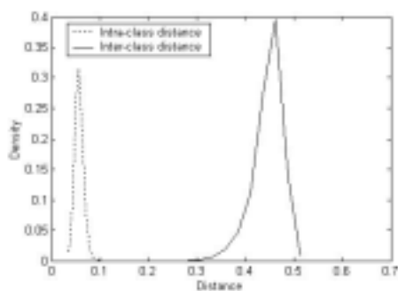
Figure 8. The intra-class and inter-class distance distribution
