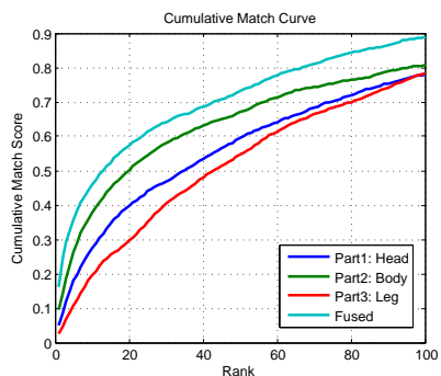
Fig. 8. The rank curves of the 3 parts and the whole image in the cross database experiment (CUHK Campus \rightarrow VIPeR).
