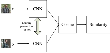
Fig. 2. The structure of the siamese convolutional neural network (SCNN). The SCNN can work in two modes: sharing parameters (General SCNN) and independent parameters (View Specific SCNN)
